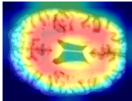
Patient 1 - \hat{\theta} = 0.01
