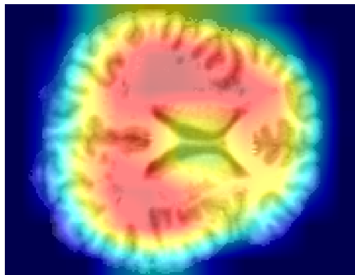
Patient 3 - \hat{\theta} = 0.17
