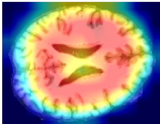
Patient 2 - \hat{\theta} = 0.05
