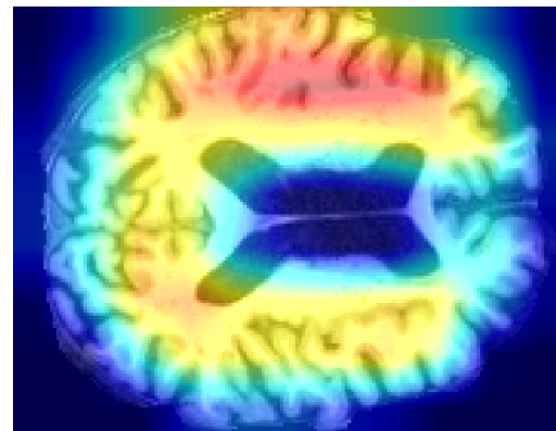
Patient 5 - \hat{\theta} = 0.86
