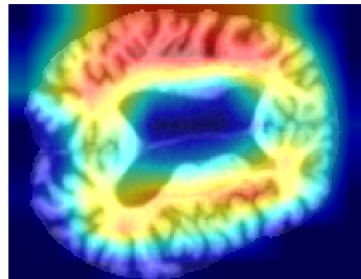
Patient 6 - \hat{\theta} = 1.84
