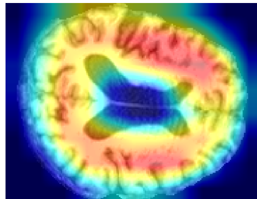
Patient 4 - \hat{\theta} = 0.32
